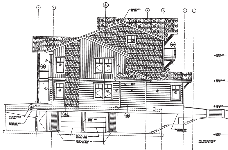
North ELEVATION
