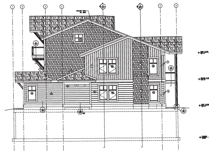
South ELEVATION
