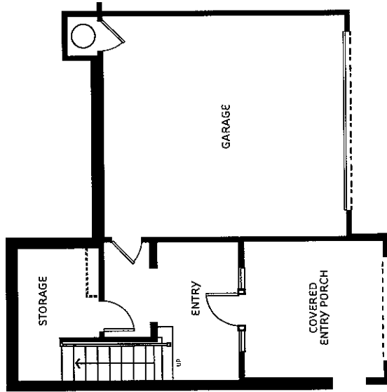
MAIN LEVEL
